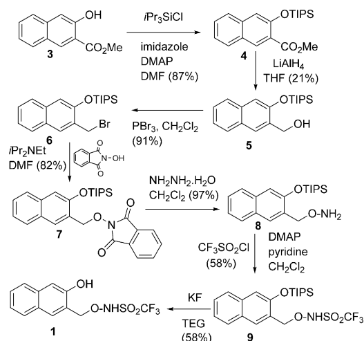
Scheme 1. Synthesis of HNO donor 1 .
