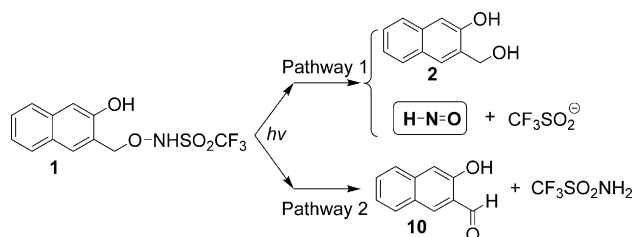
Scheme 2. Proposed pathways for the photolysis of HNO donor 1 .
